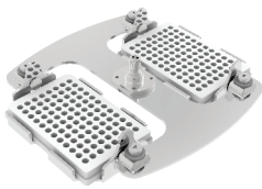
Cat. No. # LC01-L30-124 Capacity: 2 x PCR Plates RCF: 2355 g
